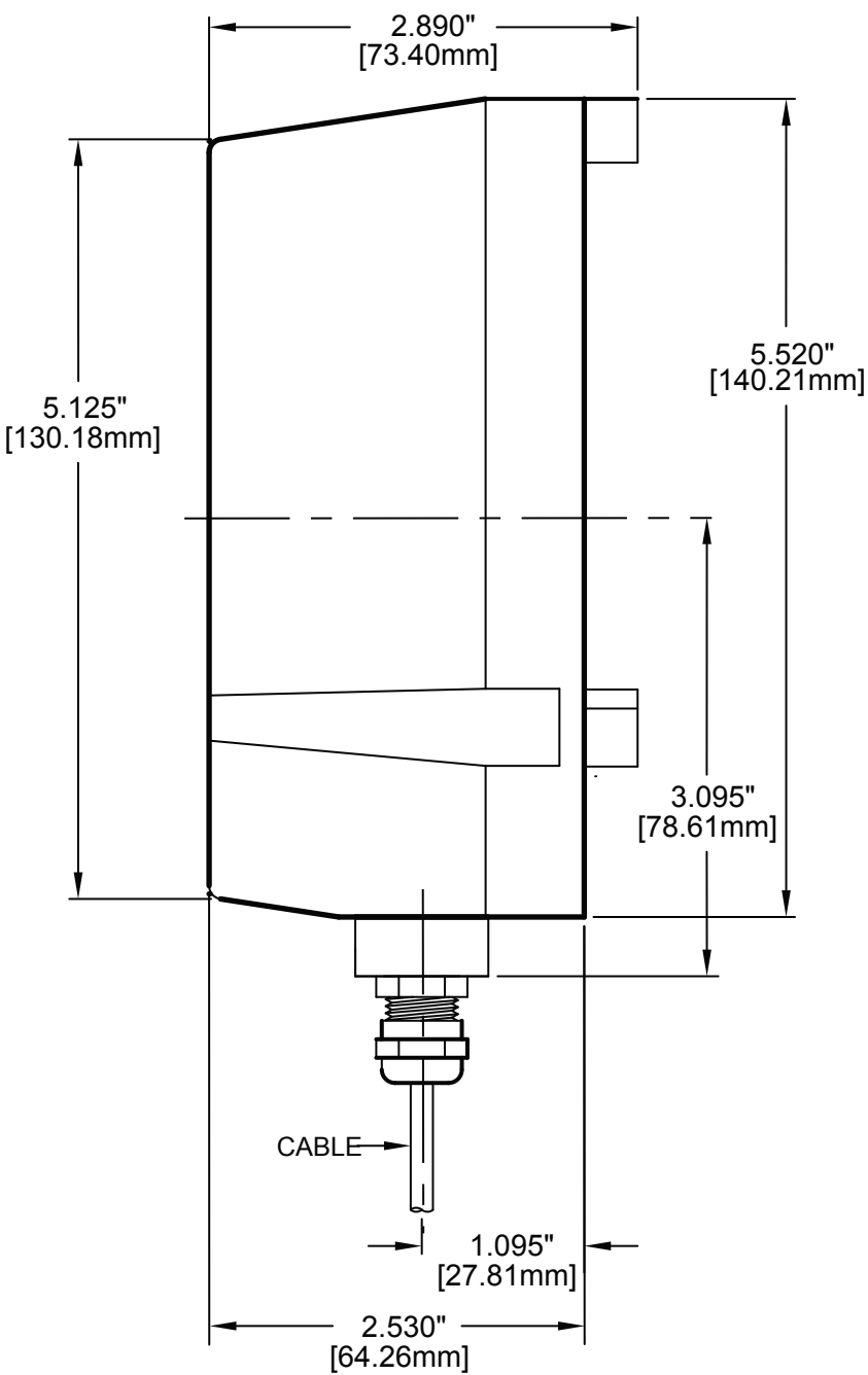
ND4RB (battery powered)
