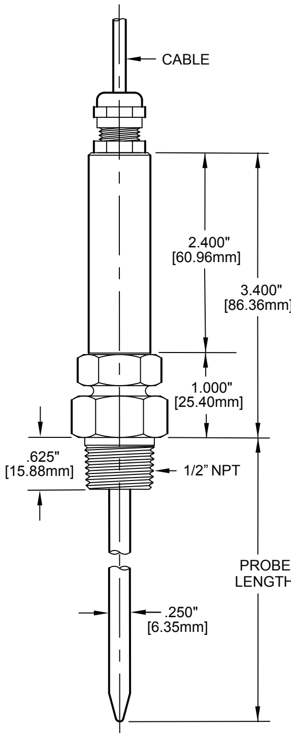
Optional 316SS pointed .250" diameter probe
