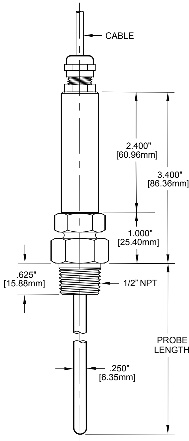
Standard 316SS blunt .250" diameter probe
