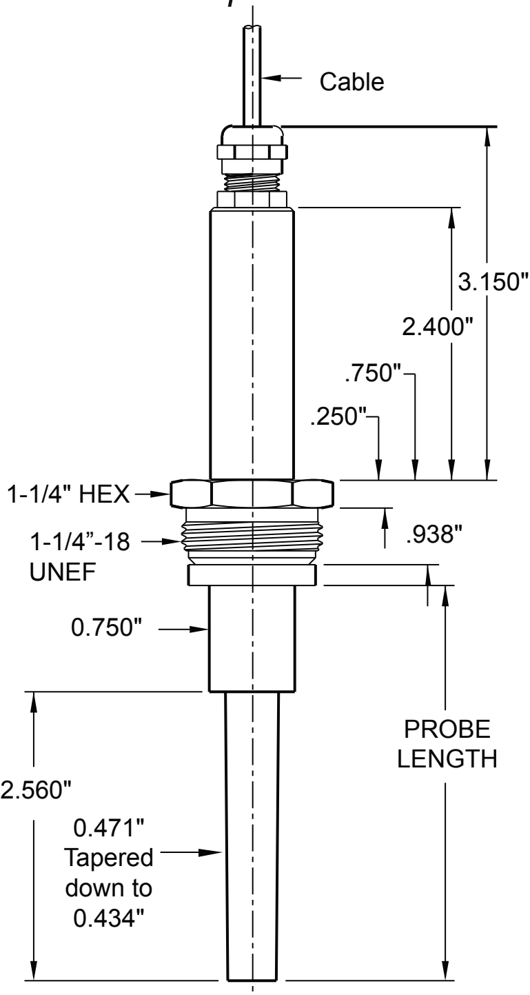
Optional 316SS 5/8" diameter probe with 7/16" tapered bulb
