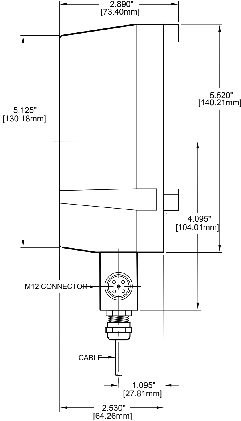
ND4RC (loop powered)
