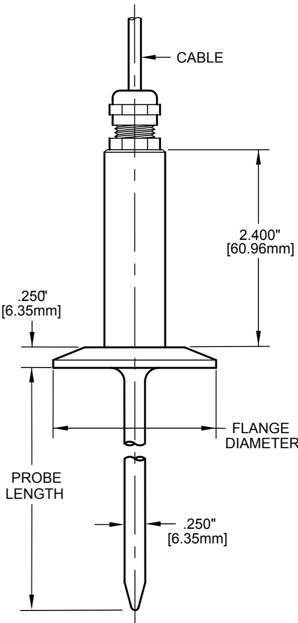
Optional 316SS pointed .250" diameter probe
