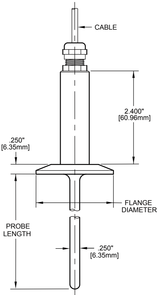
Standard 316SS blunt .250" diameter probe
