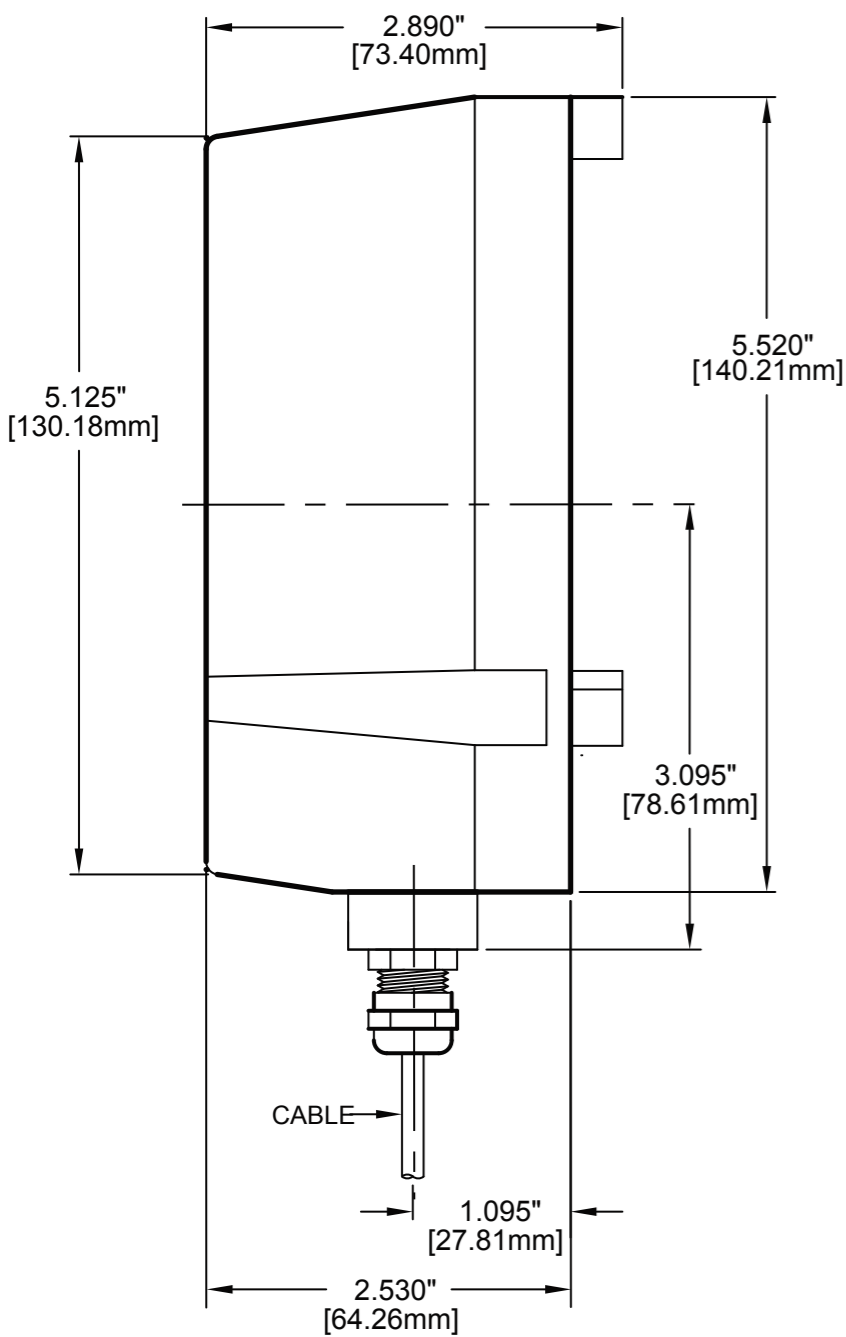
SD4RB (battery powered)
